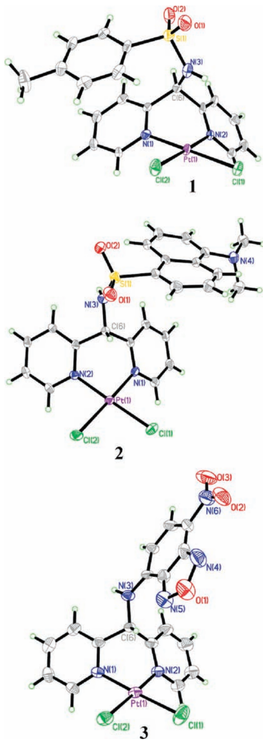
Figure 2. Molecular structures of 1–3. Thermal ellipsoids are drawn at the 50% probability level. Carbon and hydrogen atoms are not labeled. Solvent molecules of crystallization for 2 and 3 are omitted for clarity. Disorder in 3 has been omitted as well.
