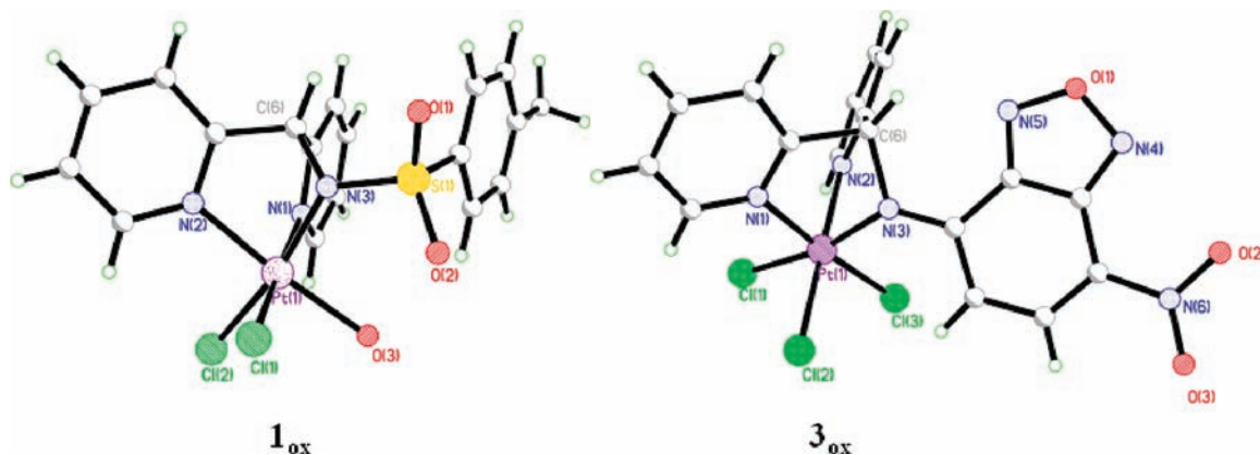
Figure 10. Ball-and-stick structures of 1_{\text{ox}} and 3_{\text{ox}} as determined by X-ray crystallography demonstrating likely atomic connectivity. Carbon and hydrogen atoms are not labeled. The hydrogen atom of O(3) in 1_{\text{ox}} was not located and is not shown.
