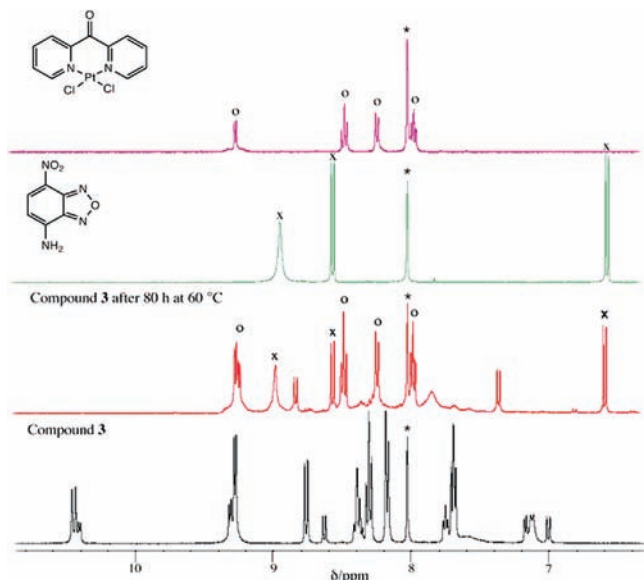
Figure 9. From bottom to top: ^1\text{H} NMR spectra of 3 , 3 after thermolysis at 60^\circ\text{C} for 80 h, NBD-NH 2 , and [Pt(dpk)Cl 2 ] in DMF- d 7 . Resonances marked with circles are assigned to [Pt(dpk)Cl 2 ], and resonances marked with crosses are assigned to NBD-NH 2 . The doublets at 8.8 and 7.3 ppm and the broad singlet at 7.8 ppm are currently unassigned. The sharp singlet at 8 ppm in all spectra marked by an asterisk is from the solvent.
