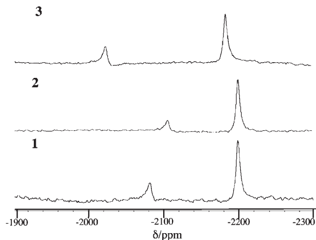
Figure 5. ^{195}\text{Pt} NMR spectra of 1 (bottom), 2 (middle), and 3 (top) in DMF- d_7 . Signals are observed for both the exo (major) and endo (minor) conformers.
