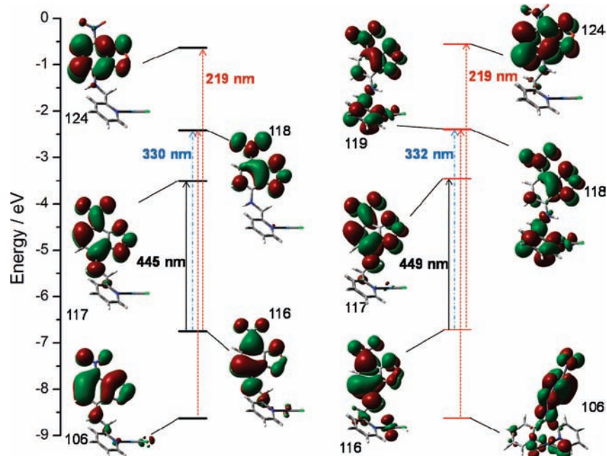
Figure 8. MOs that contribute to the main electronic absorption bands for both the exo (left) and the endo (right) conformers. Arrows indicate the calculated electronic transitions. MO surfaces are shown with a contour value of 0.02 au.
