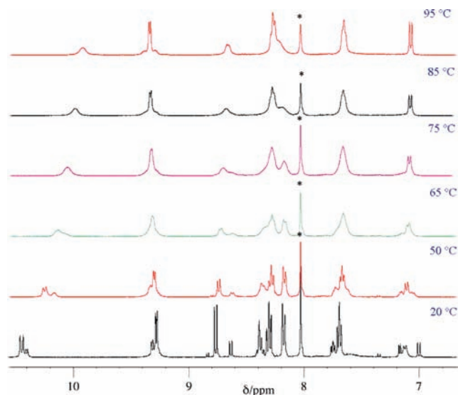
Figure 4. VT ^1\text{H} NMR spectra of 3 in \text{DMF-}d_7 . As the temperature is elevated above 50 ^\circ\text{C} , the distinct resonances for the exo and endo conformers coalesce. For full peak assignment of 3 at 20 ^\circ\text{C} , see Figure S12 in the SI. VT-NMR spectra for 1 and 2 are provided in Figures S4 and S5 in the SI. The singlet at 8 ppm marked by an asterisk is from the solvent.
