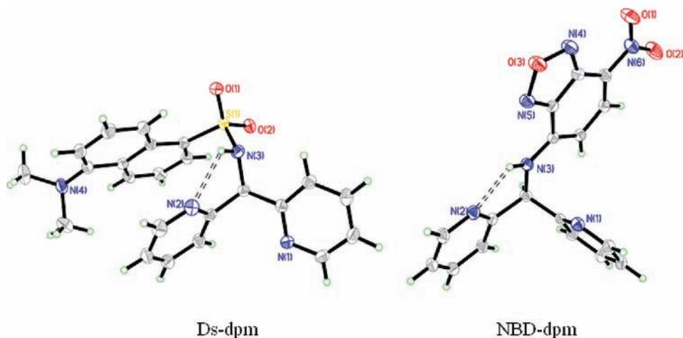
Figure 1. Molecular structures of Ds-dpm (left) and NBD-dpm (right). Thermal ellipsoids are drawn at the 50% probability level. Carbon (gray) and hydrogen (green circles) atoms are not labeled.
