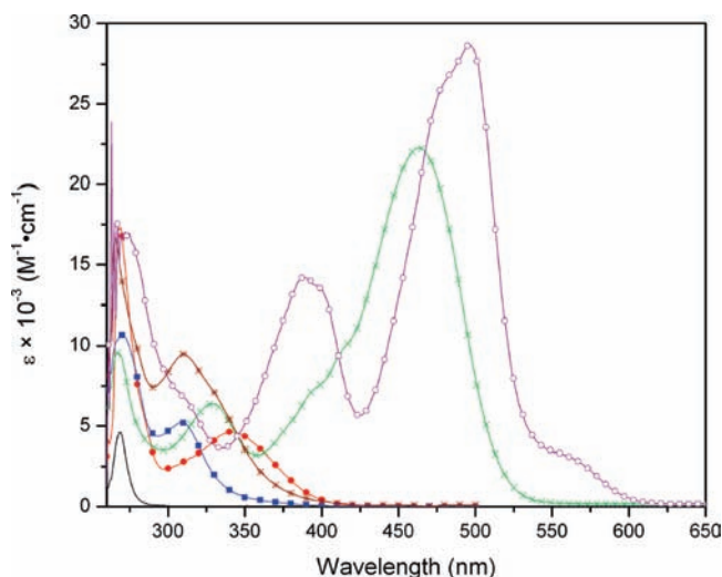
Figure 6. UV-vis absorption spectra for Ts-dpm (—), Ds-dpm (red ●), NBD-dpm (green ×), 1 (blue ■), 2 (maroon *), and 3 (purple ○) in DMF at room temperature.
