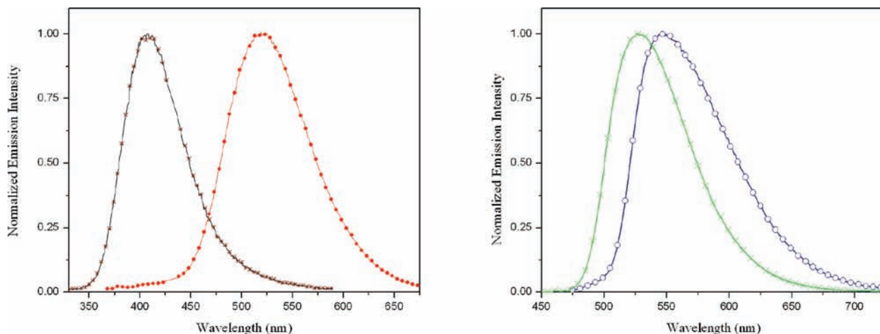
Figure 7. Room temperature normalized emission spectra of (left) Ds-dpm (red ●) and 2 (maroon *) and (right) NBD-dpm (green ×) and 3 (blue ○) in DMF. Spectra were obtained by exciting compounds at their wavelengths of maximum absorption.
